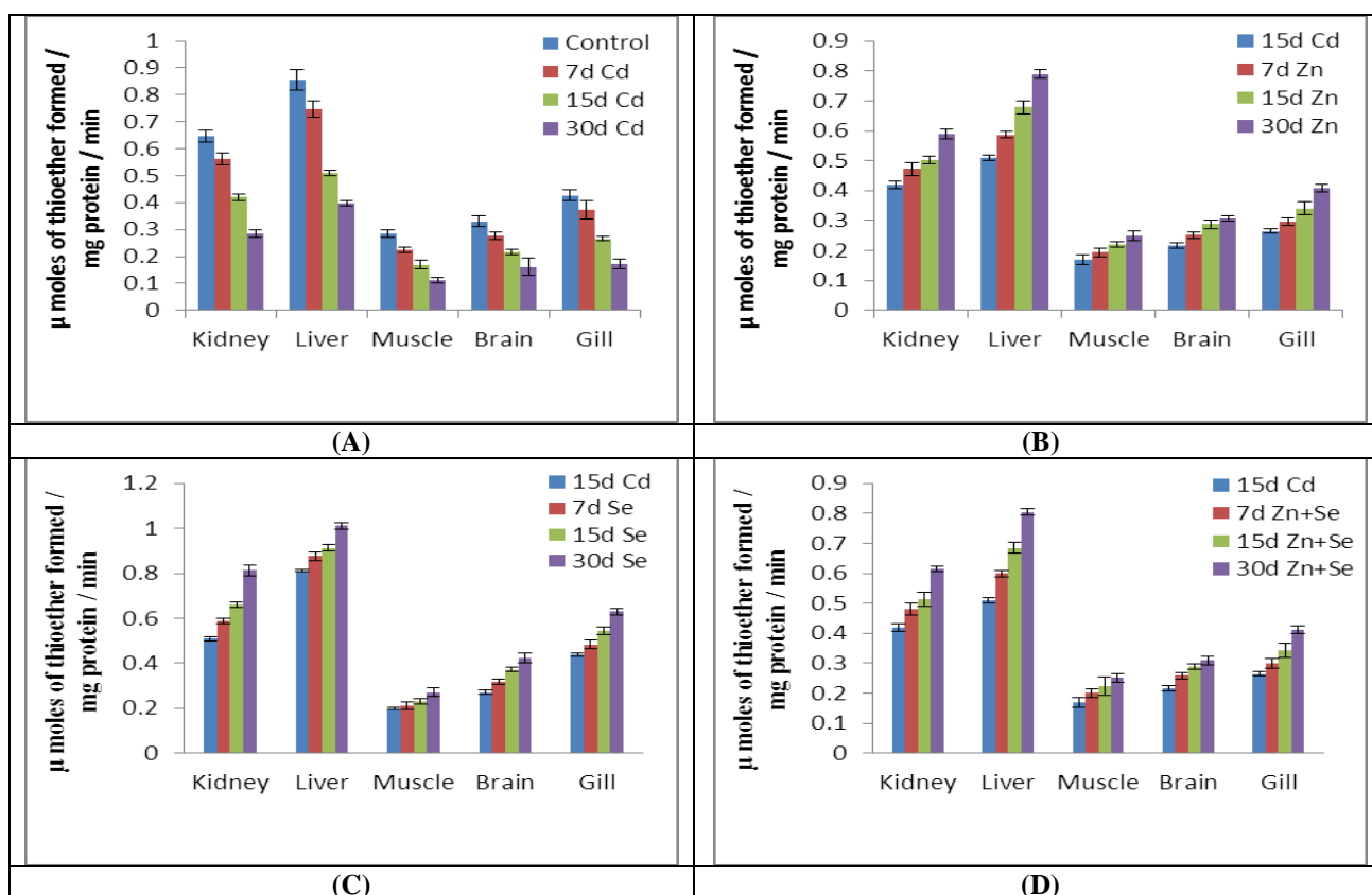
Fig.5: (A). Changes in GST activity in different tissues of Cd exposed O. mossambicus . (B). Changes in GST activity in different tissues of Cd exposed O. mossambicus under Zn supplementation. (C). Changes in GST activity in different tissues of Cd exposed O. mossambicus under Se supplementation. (D). Changes in GST activity in different tissues of Cd exposed O. mossambicus under Zn+ Se supplementation. Values are expressed as mean \pm SD (n = 6 rats in each group), Statistical significance was evaluated by one-way analysis of variance (ANOVA) and the Duncan's Multiple Range Test (DMRT). All experimental mean values are significant at P<0.05 level over control. 15d Cd treated rats considered as control for supplementation groups (B, C, D).
