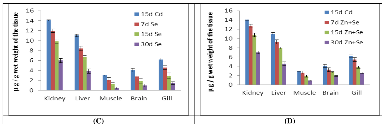
Fig. 1: (A). Cd Bio-accumulation levels in different tissues of Cd exposed O. mossambicus . (B). Changes in Cd Bio-accumulation levels in different tissues of Cd exposed O. mossambicus under Zn supplementation. (C). Changes in Cd Bio-accumulation levels in different tissues of Cd exposed O. mossambicus under Se supplementation. (D). Changes in Cd Bio-accumulation levels in different tissues of Cd exposed O. mossambicus under Zn+Se supplementation. Values are expressed as mean±SD (n = 6 rats in each group), Statistical significance was evaluated by one-way analysis of variance (ANOVA) and the Duncan's Multiple Range Test (DMRT). All experimental mean values are significant at P<0.05 level over control. 15d Cd treated rats considered as control for supplementation groups (B, C, D).
