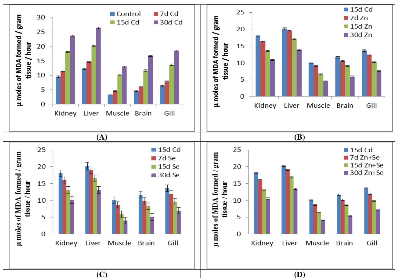
Fig. 2: (A). Changes in LPO levels in different tissues of Cd exposed O. mossambicus . (B). Changes in LPO levels in different tissues of Cd exposed O. mossambicus under Zn supplementation. (C). Changes in LPO levels in different tissues of Cd exposed O. mossambicus under Se supplementation. (D). Changes in LPO levels in different tissues of Cd exposed O. mossambicus under Zn+Se supplementation. Values are expressed as mean±SD (n = 6 rats in each group), Statistical significance was evaluated by one-way analysis of variance (ANOVA) and the Duncan's Multiple Range Test (DMRT). All experimental mean values are significant at P<0.05 level over control. 15d Cd treated rats considered as control for supplementation groups (B, C, D).
