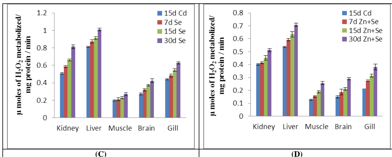
Fig.4: (A). Changes in CAT activity in different tissues of Cd exposed O. mossambicus . (B). Changes in CAT activity in different tissues of Cd exposed O. mossambicus under Zn supplementation. (C). Changes in CAT activity in different tissues of Cd exposed O. mossambicus under Se supplementation. (D). Changes in CAT activity in different tissues of Cd exposed O. mossambicus under Zn+ Se supplementation. Values are expressed as mean \pm SD (n = 6 rats in each group), Statistical significance was evaluated by one-way analysis of variance (ANOVA) and the Duncan's Multiple Range Test (DMRT). All experimental mean values are significant at P<0.05 level over control. 15d Cd treated rats considered as control for supplementation groups (B, C, D).
