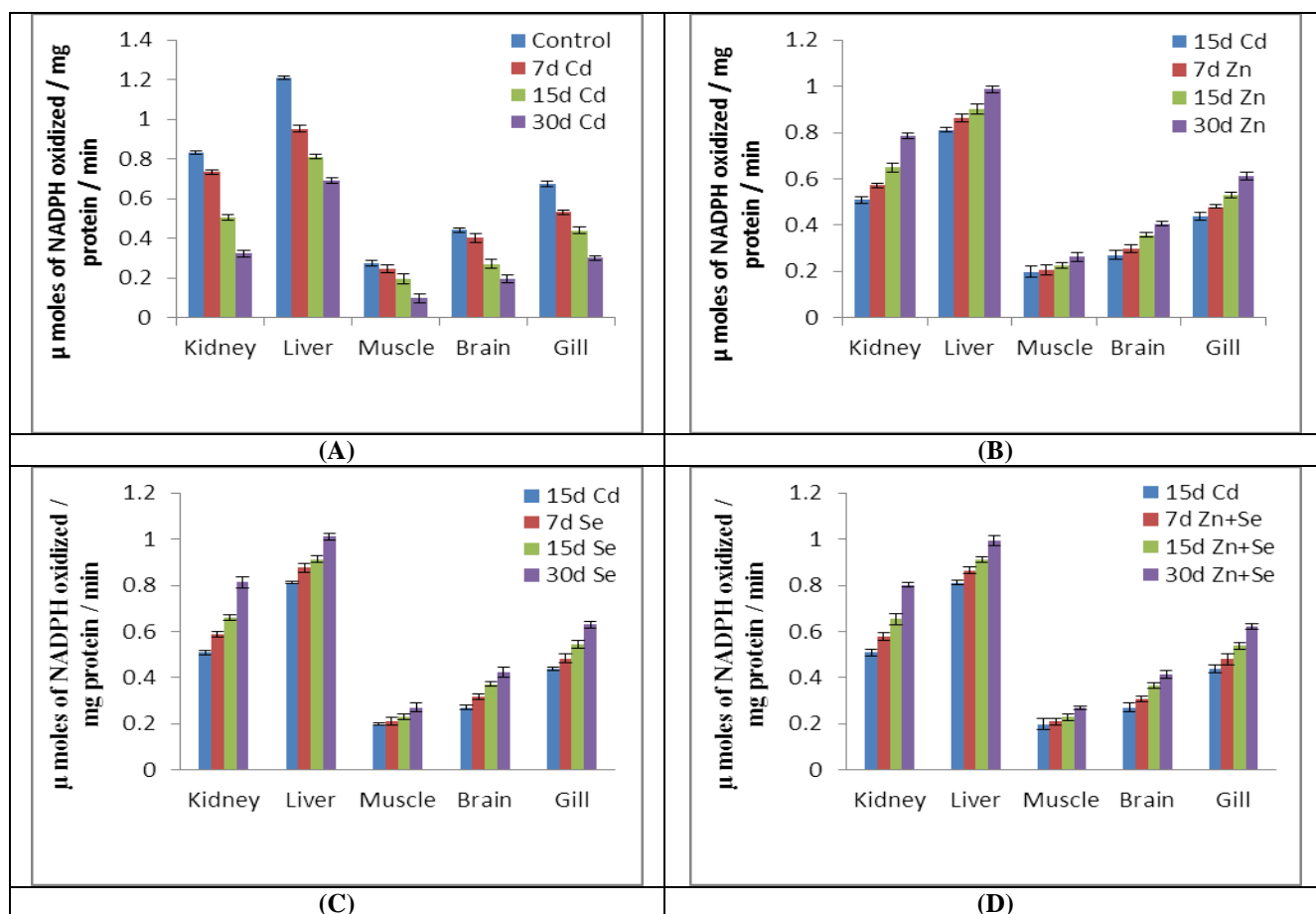
Fig. 6: (A). Changes in GPx activity in different tissues of Cd exposed O. mossambicus . (B). Changes in GPx activity in different tissues of Cd exposed O. mossambicus under Zn supplementation. (C). Changes in GPx activity in different tissues of Cd exposed O. mossambicus under Se supplementation. (D). Changes in GPx activity in different tissues of Cd exposed O. mossambicus under Zn+ Se supplementation. Values are expressed as mean \pm SD (n = 6 rats in each group), Statistical significance was evaluated by one-way analysis of variance (ANOVA) and the Duncan's Multiple Range Test (DMRT). All experimental mean values are significant at P<0.05 level over control. 15d Cd treated rats considered as control for supplementation groups (B, C, D).
