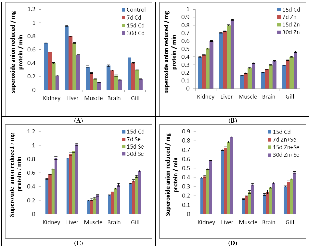
Fig. 3: (A). Changes in SOD activity in different tissues of Cd exposed O. mossambicus . (B). Changes in SOD activity in different tissues of Cd exposed O. mossambicus under Zn supplementation. (C). Changes in SOD activity in different tissues of Cd exposed O. mossambicus under Se supplementation. (D). Changes in SOD activity in different tissues of Cd exposed O. mossambicus under Zn+ Se supplementation. Values are expressed as mean \pm SD (n = 6 rats in each group), Statistical significance was evaluated by one-way analysis of variance (ANOVA) and the Duncan's Multiple Range Test (DMRT). All experimental mean values are significant at P < 0.05 level over control. 15d Cd treated rats considered as control for supplementation groups (B, C, D).
