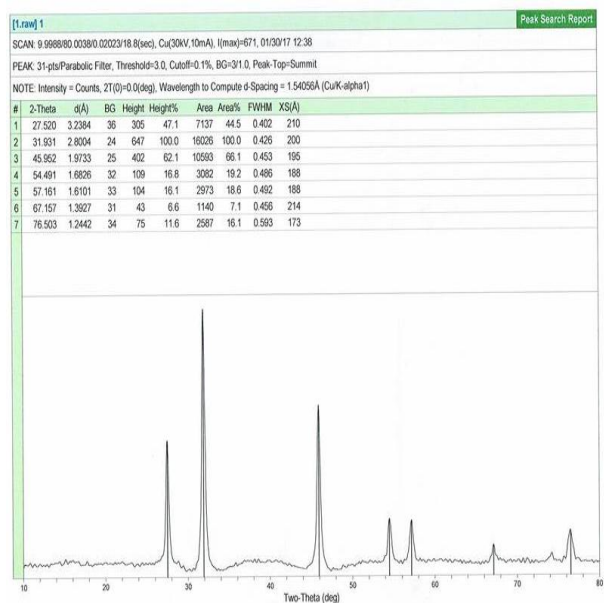
Fig. 2: XRD analysis of Biosynthesized nanoparticles using S.boulardii (average diameter 19.92nm).
