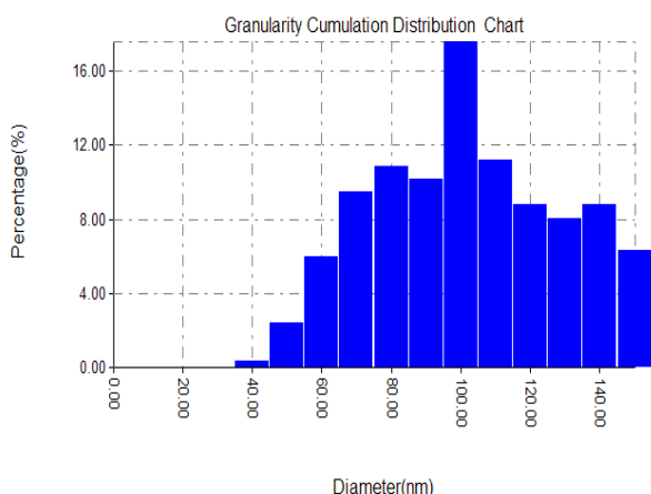
Fig. 5: Atomic Force Microscopic analysis of biosynthesized silver nanoparticle from S.boulardii (Average Diameter: 97.44 nm).
