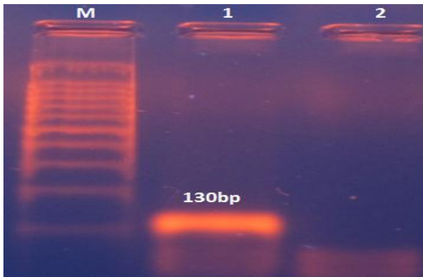
Fig. 1: Agarose gel electrophoresis (1.5% Agarose gel, 75 volts to 1 hours) for PCR product (130bp) of (CAG) n microsatellite repeat at locus YLR177w of S.boulardii Lane (M) :size marker (200 bp DNA Even Ladder); Lane 1 PCR product, Lane 2: negative control.
