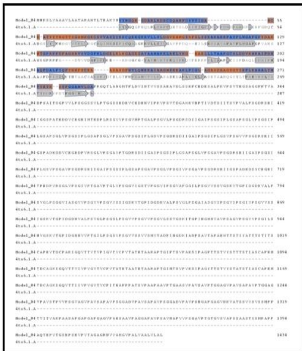
Fig. 6: Target-Template Alignment showed overall 254 templates out of them the selected template Chitinase Chi A1 (4tx6.1.A) were used to build this model.
