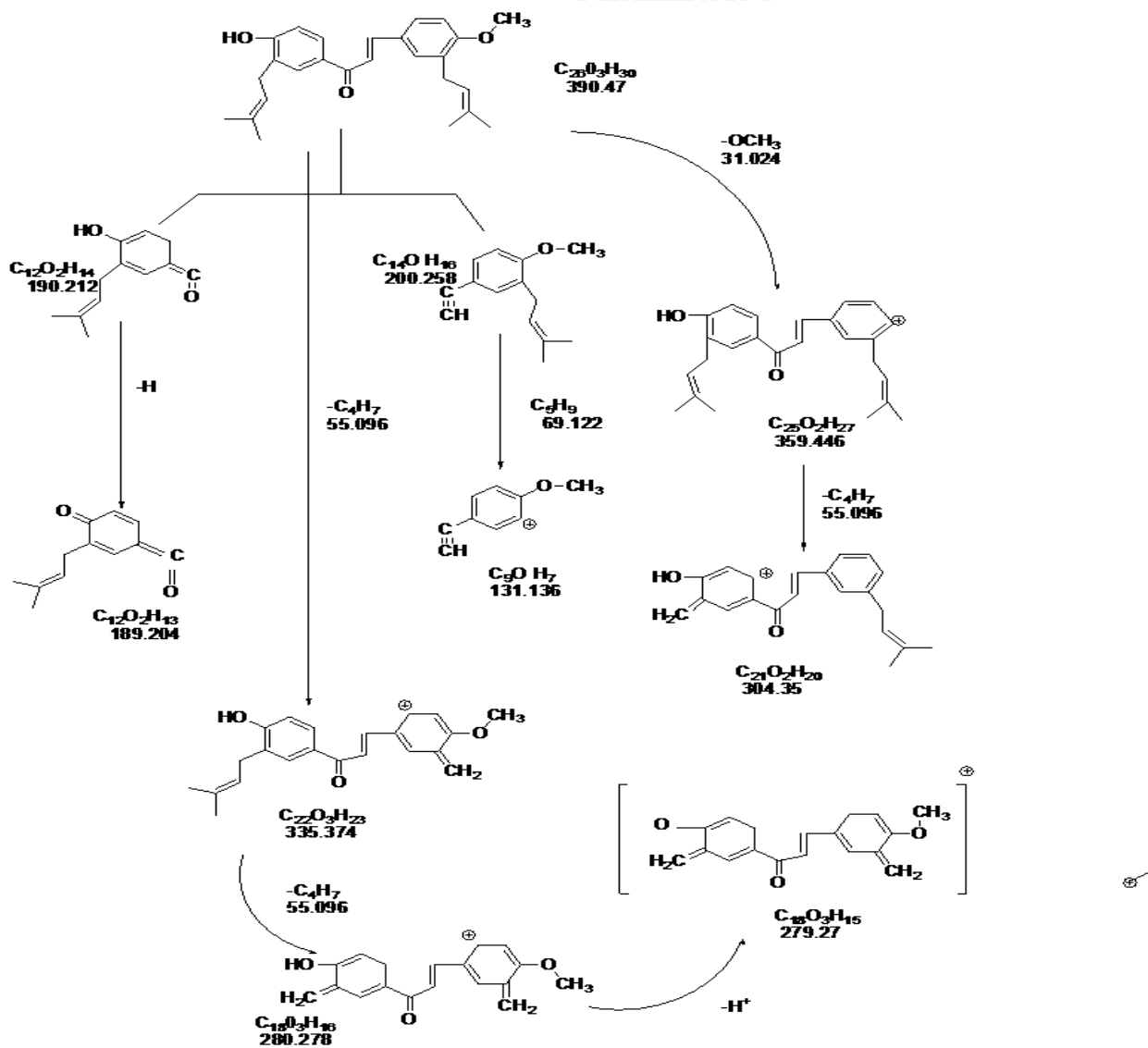
Scheme 2 Part 1
