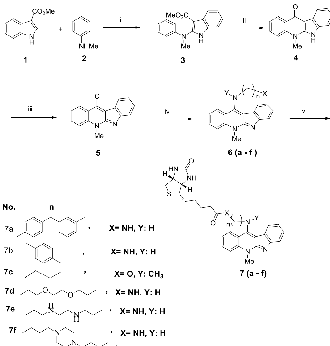
Scheme 1: Reagents and conditions: (i) a, N-Chlorosuccinimide, 1,4-dimethylpiperazine, \text{CH}_2\text{Cl}_2 , ^\circ\text{C} , 2 h; b, trichloroacetic acid, RT, 2 h; (ii) diphenyl ether, reflux, 1-3 h; (iii) \text{POCl}_3 , toluene, reflux. 6-12 h; (iv) appropriate amine, DMF, 135^\circ\text{C} .
