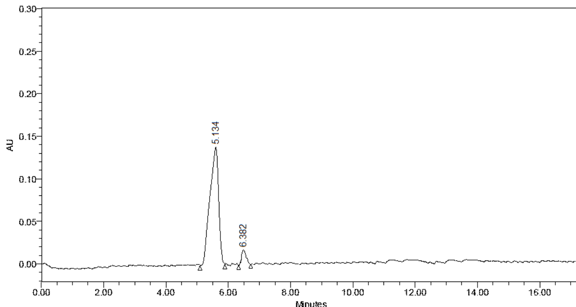
Fig. 8: Chromatogram showing the degraded products in Oxidative degradation.
