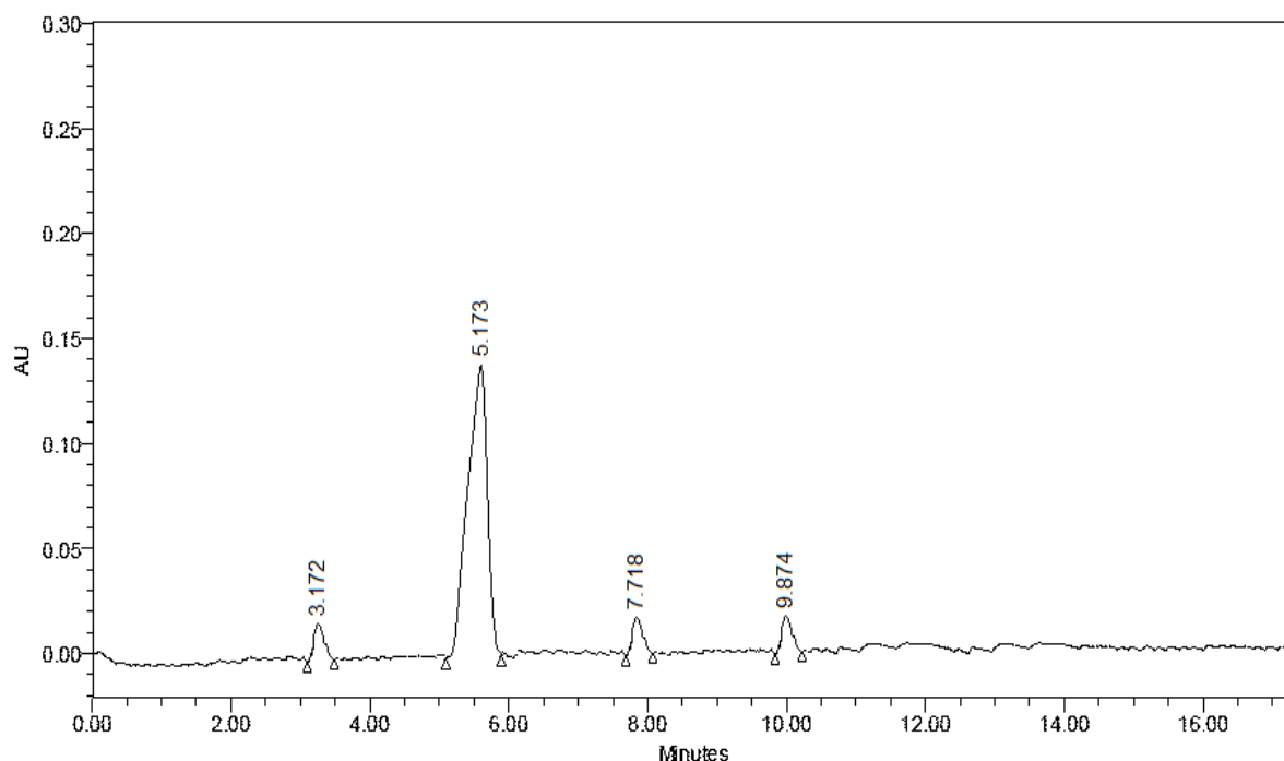
Fig. 5: Chromatogram showing the degraded products in Acidic degradation.
