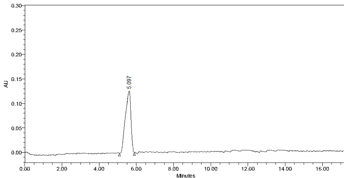
Fig. 4: Chromatogram Showing accuracy results.
