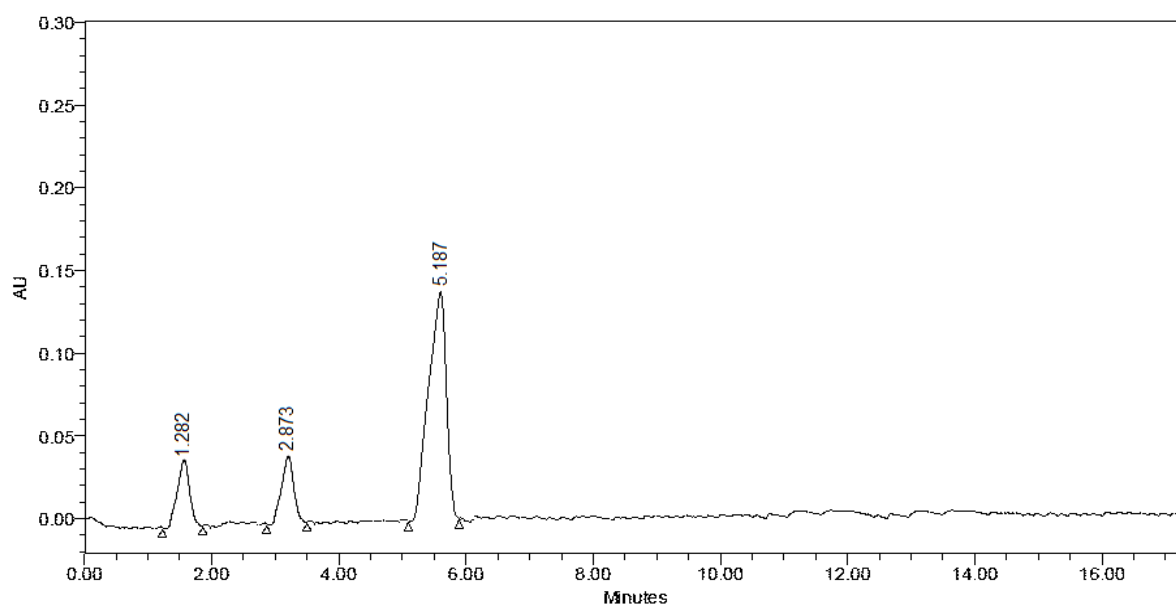
Fig. 7: Chromatogram showing the degraded products in Wet heat degradation.
