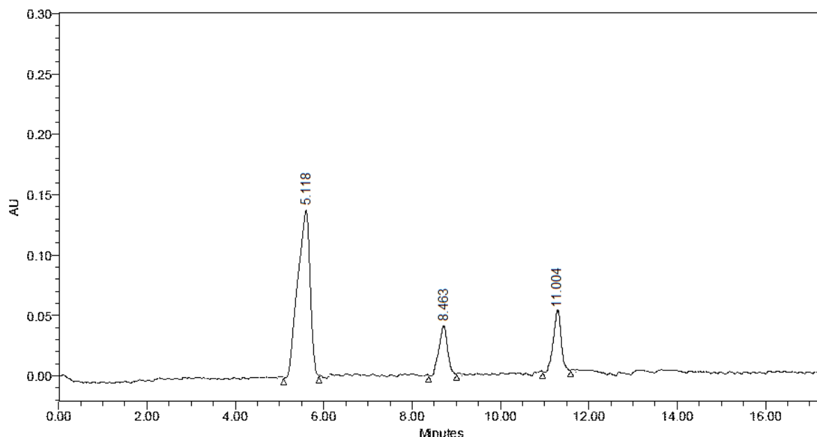
Fig. 6: Chromatogram showing the degraded products in Basic degradation.
