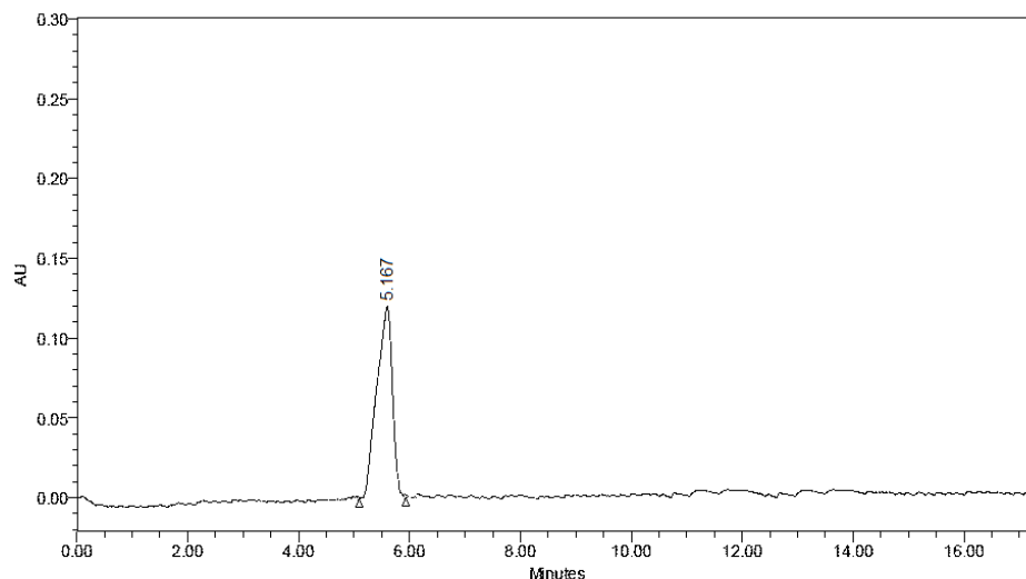
Fig. 2: Optimized chromatogram of Fluorometholone and internal standard using mobile phase of Acetonitrile with buffer 0.5M potassium dihydrogen orthophosphate (35: 65%v/v).
