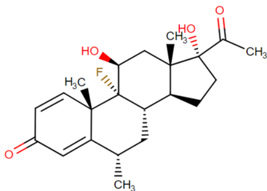
Fig. 1: Structure of Fluorometholone.
